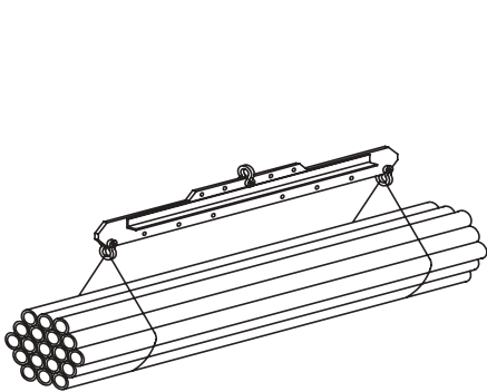
2 Point Lift
