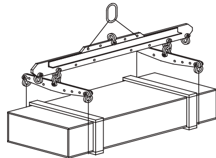
4 Point Lift
