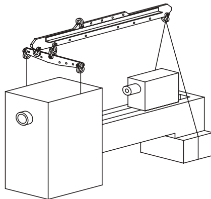
3 Point Lift
